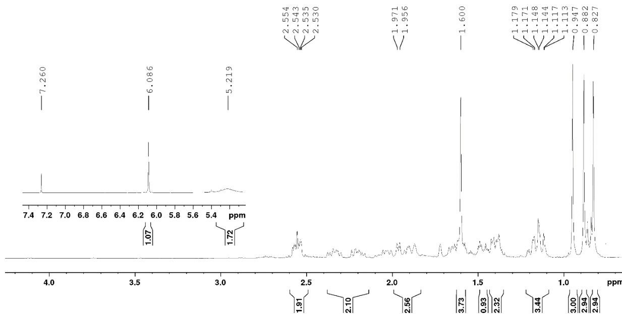
Figure 1. 1 H NMR spectrum of 2-amino-4-(15,16-di-norlabd-8(9)-en-13-on)-1,3-thiazole.
