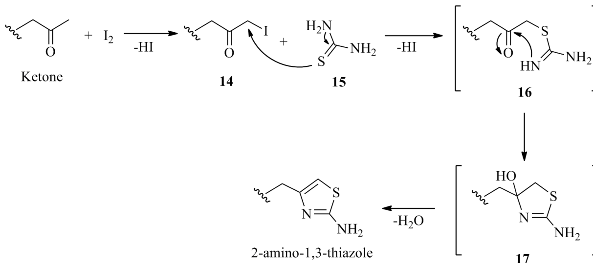
Scheme 3. Proposed mechanism for the synthesis of 2-amino-1,3-thiazole fragment.
