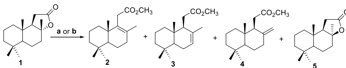
Scheme 1. Syntheses of bicyclohomofarnesenic methyl esters 2-4 from (+)-sclareolide ( 1 ).
