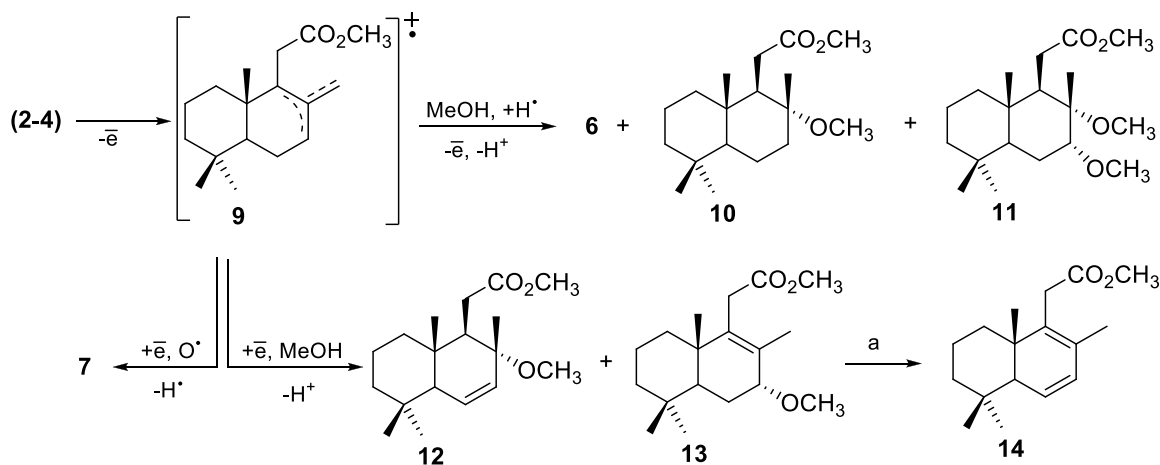
Scheme 3. Minor compounds from anodic oxidation of mixture of methyl esters 2-4 .
