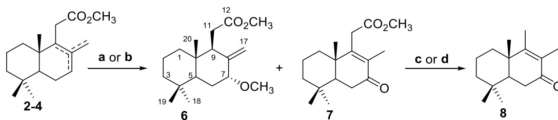
Scheme 2. Syntheses of ketoester 7 and drimenone 8 .
