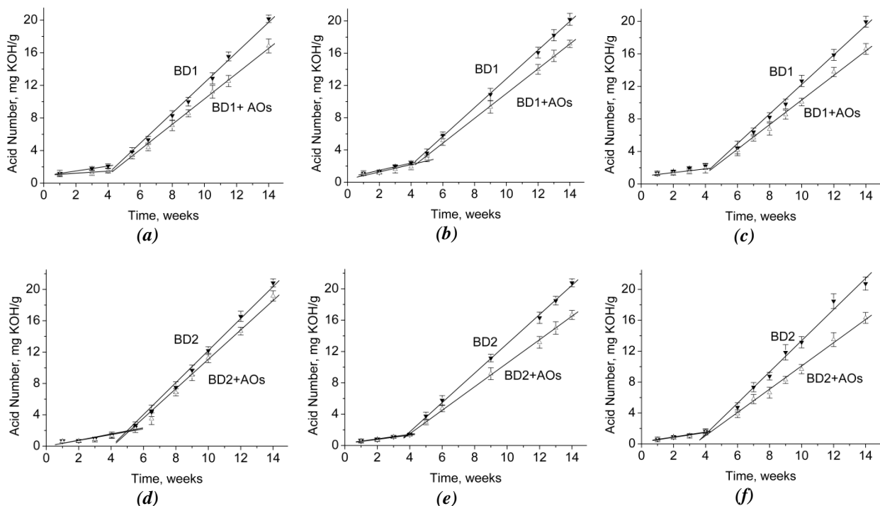
Figure 5. Acid number for BD and BD+AOs samples vs time of oxidation at 43°C. AOs are extracts from C. japonica (a, d) and D. antarctica (b, e) plants and from defatted S. marianum seedcake (c, d).
